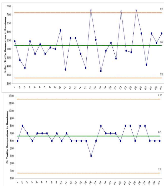
Figure 5 Six Sigma Control Chart X-Bar R Chart
