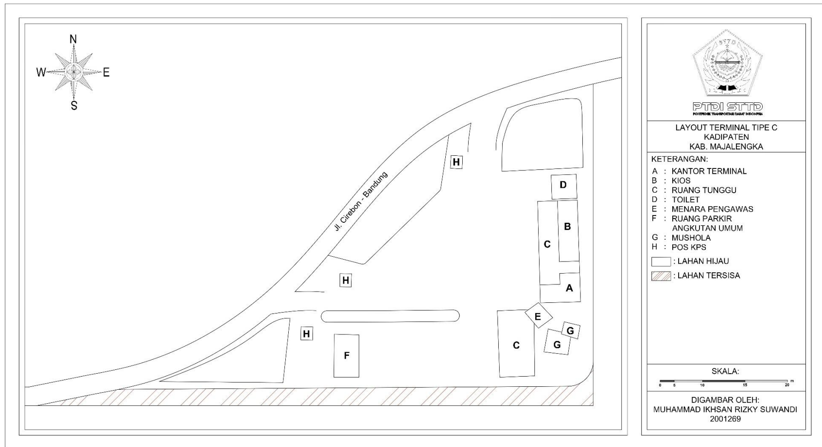
Gambar II. 13 Layout Eksisting Terminal Kadipaten
