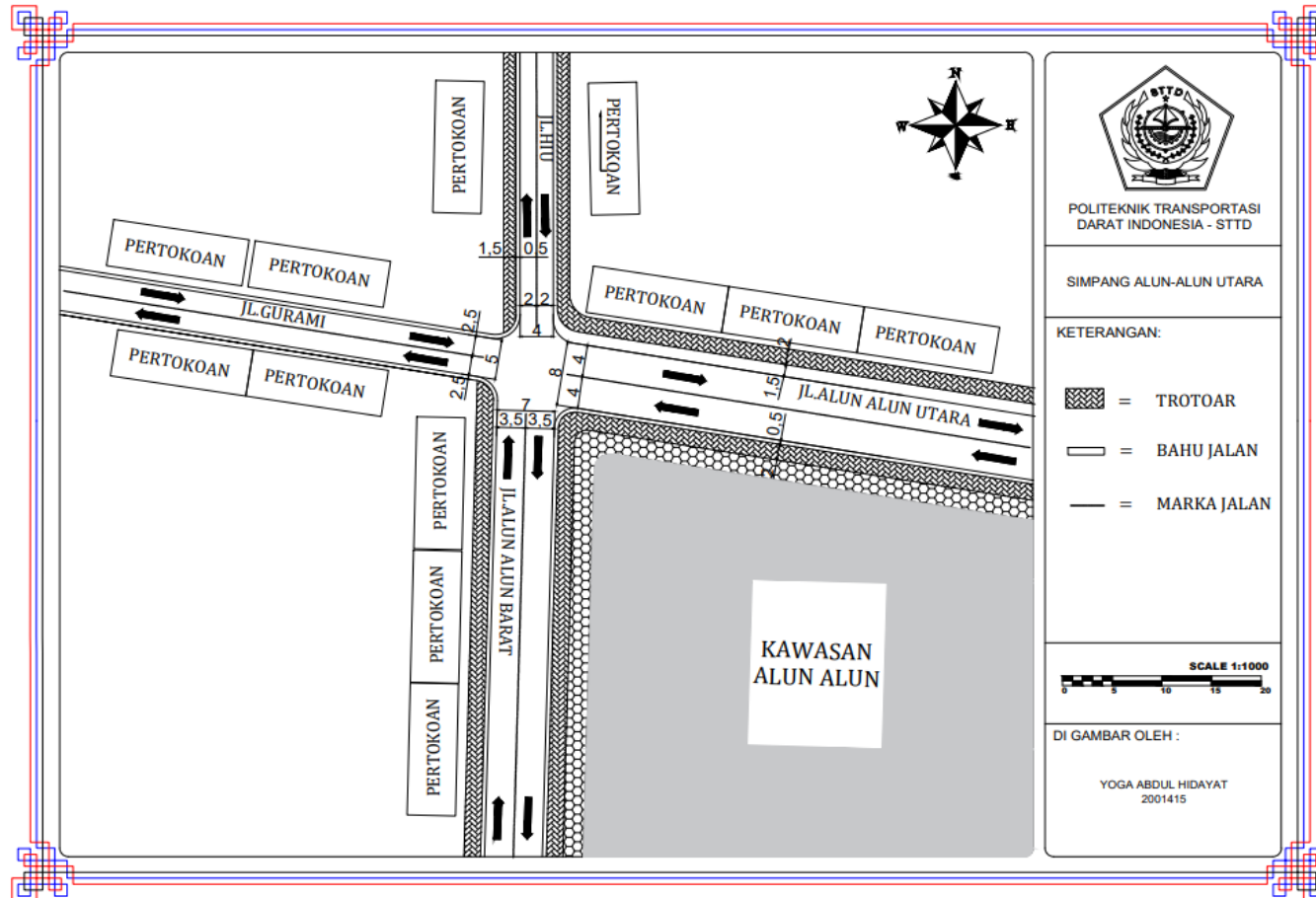
Gambar II. 3 Layout Simpang Alun-alun Utara
