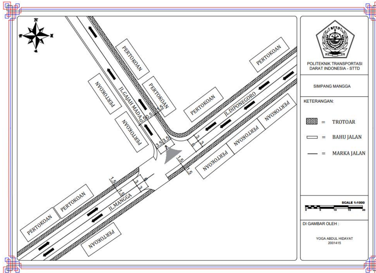
Gambar II. 7 Layout Simpang Mangga
