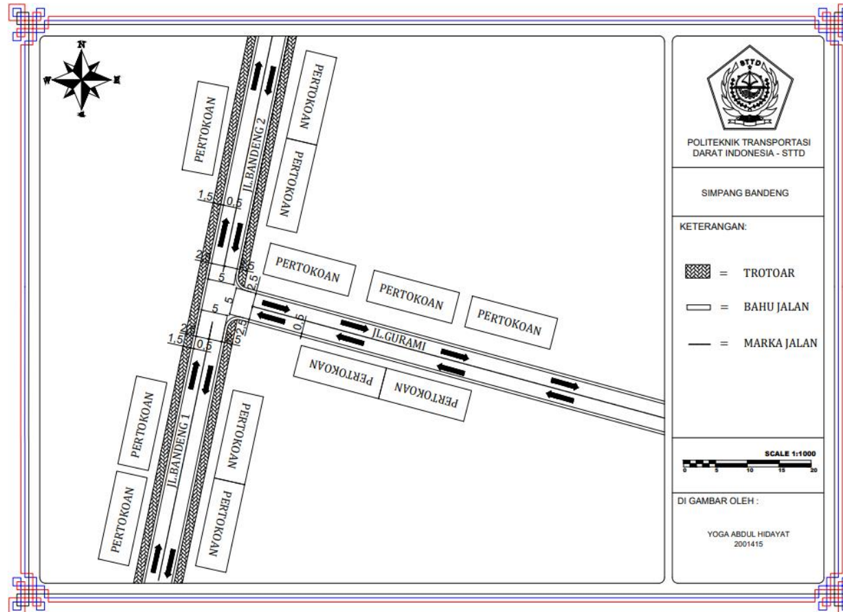
Gambar II. 9 Layout Simpang Bandeng
