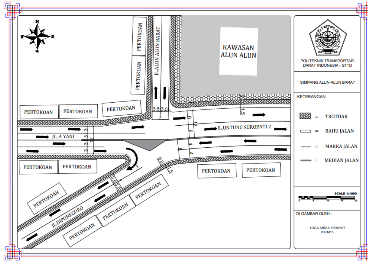
Gambar II. 6 Layout Simpang Alun-alun Barat
